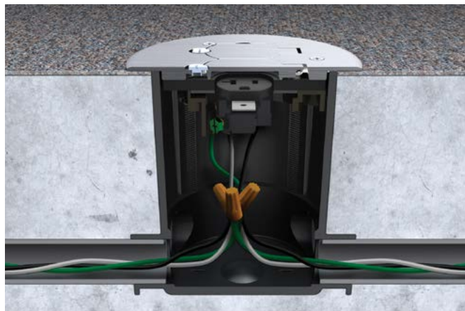
Ratchet-Pro Series Floor Box can be used in both on grade and above grade concrete construction.
