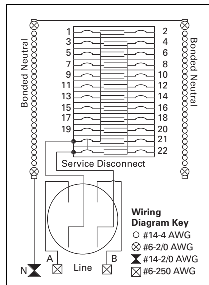
Figure 3. Catalog Numbers – CMBE2222B125BS, CMBE2222B125BF, CMBE2222B100BS and CMBE2222B100BF
