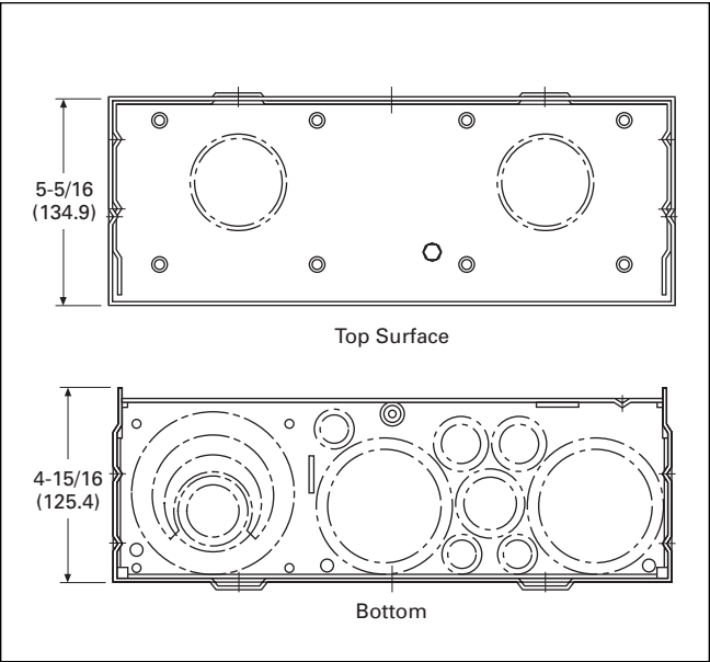
Figure 40. Knockouts for Stucco and Surface Units Catalog Numbers – MBE1224B100TS, MBE1224B125TS, MBE816P200TS, MBE816P200TSU, MBE2040P200TS, MBE1212L200TS, CMBE1212L200TS, CMB1212P200BTS, CMB1212P200BTSD, CMB1212B200BTS, CMB1212B200BTSD, MB1212L200BTS, MB1212L200BTSD, CMB1212L200BTS and CMB1212L200BTSD
