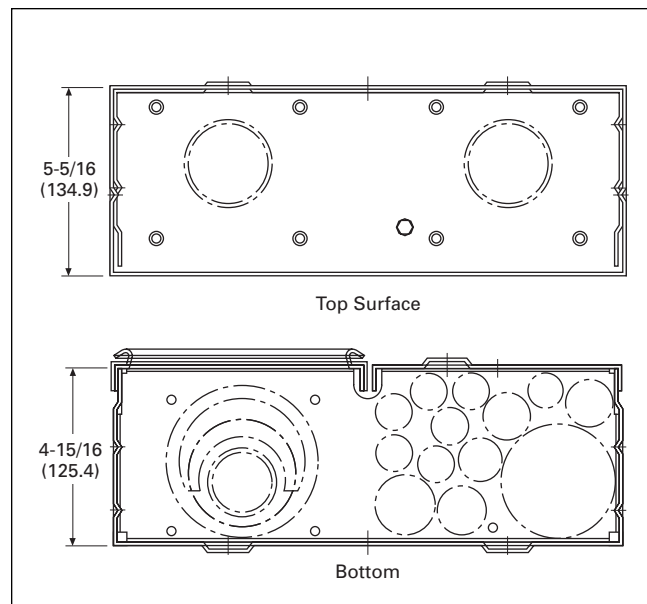
Figure 38. Knockouts for Stucco and Surface Units Catalog Numbers – CMBB200BTS, CMBE24L125BTS, CMB24L125BTS, CMBE24L200BTS, CMBE200BTS, CMBE150BTS, CMBE88B150BTS, CMBE88B200BTS, MBE24L125BTS, MBE24L200BTS, MBE48B150BTS, MBE48B200BTS, MBE88B150BTS, MBE88B200BTS, MBE150BTS, MBE200BTS, MBEP200BTS, MBE1224B100BTS, MBE1224B125BTS, CMB88B150BTS, CMB88B200BTS and MB48B200BTS
