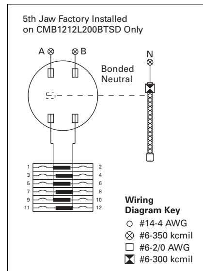
Figure 27. Catalog Numbers – CMB1212L200BTSD and CMB1212L200BTS
