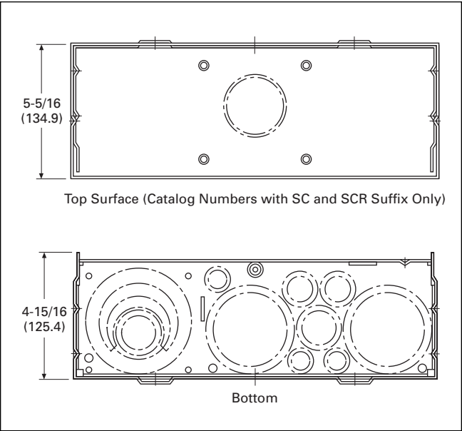
Figure 43. Knockouts for Non-EUSERC Units Catalog Numbers – MBB150BTSCR, MBB200BTSCR, MBP200BTSCR, MBB150BTSC and MBB200BTSC
