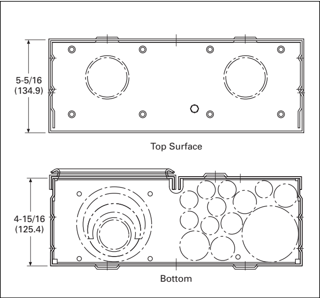
Figure 36. Knockouts for Stucco and Surface Units Catalog Numbers – CMBE3242B150BS, CMBE3242B200BS, CMBE3242B225BS, CMBE2222B100BS, CMBE2222B125BS, CMBE1212L200BS, MBE2040B200BS, MBE2040B150BS, MBE1428B100BS, MBE1428B125BS, MBE1212L200BS, MBE1836B125BS, CMB3242B150BS and CMB3242B200BS
