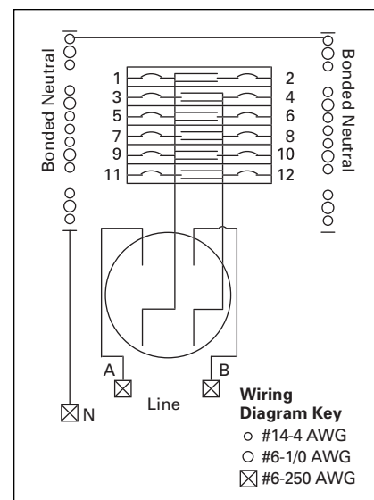
Figure 4. Catalog Numbers – CMBE1212L200BS and CMBE1212L200BF
