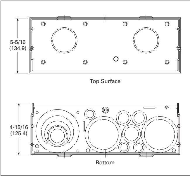
Figure 42. Knockouts for Non-EUSERC Units Catalog Numbers – MBB200BTS, MBP200BTS, MB816P200BTS, MB816P200BTSCU, MB816B200BTS, MB816B200BTSCU, MB2040P200BTS, MB2040B200BTS, MBP200SD, MB816P200STD and MB2040P200SD
