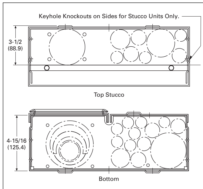
Figure 37. Knockouts for Stucco and Surface Units Catalog Numbers – CMBE24L200BTF, CMBE24L125BTF, CMBE200BTF, CMBE150BTF, CMBE88B150BTF, CMBE88B200BTF, MBE24L125BTF, MBE24L200BTF, MBE48B150BTF, MBE48B200BTF, MBE88B150BTF, MBE88B200BTF, MBE150BTF, MBE200BTF, MBE1224B100BTF and MBE1224B125BTF
