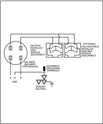
Figure 62. Type BR Wiring Diagram 10
