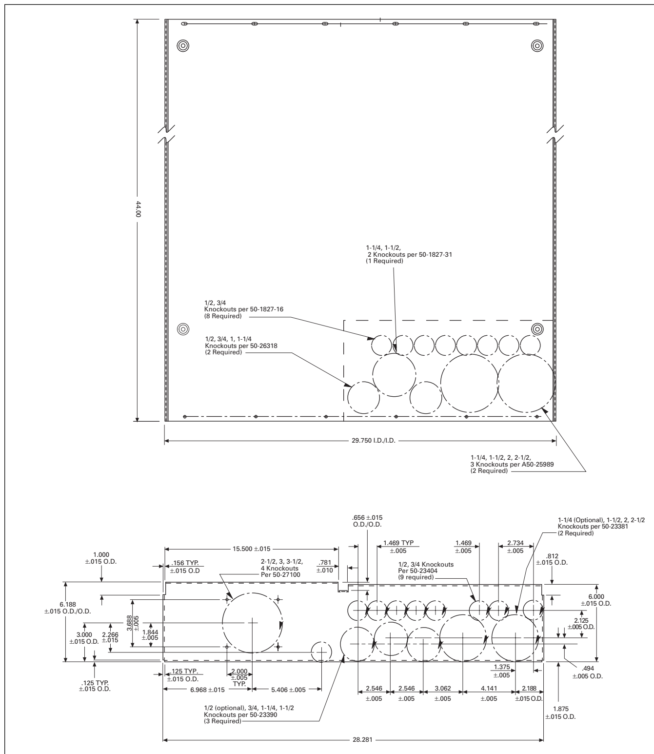
Figure 52. House Panel Dimensions and Knockouts
