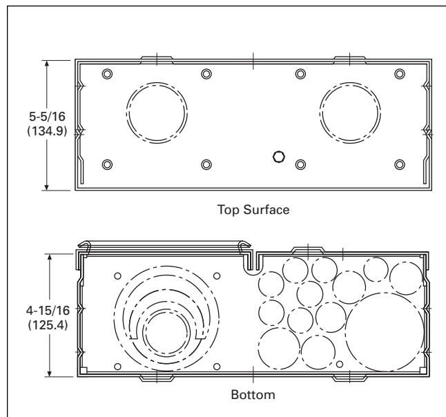
Figure 38. Knockouts for Stucco and Surface Units Catalog Numbers – CMBB200BTS, CMBE24L125BTS, CMB24L125BTS, CMBE24L200BTS, CMBE24L200BTS, CMBE48B150BTS, CMBE88B150BTS, CMBE88B200BTS, CMBE24L125BTS, CMBE24L200BTS, MBE48B150BTS, MBE48B200BTS, MBE88B150BTS, MBE88B200BTS, MBE150BTS, MBE200BTS, MBEP200BTS, MBE1224B100BTS, MBE1224B125BTS, CMB88B150BTS, CMB88B200BTS and MB48B200BTS
