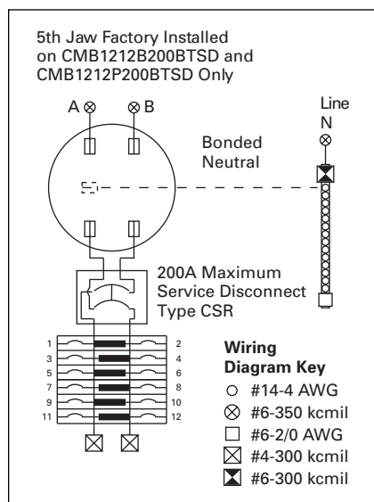
Figure 24. Catalog Numbers – CMB1212B200BTS and CMB1212B200BTSD
