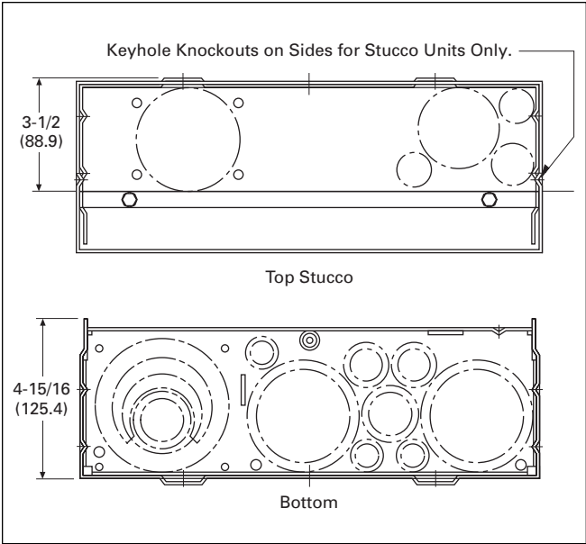
Figure 39. Knockouts for Stucco and Surface Units Catalog Numbers – MBE1224B100TF, MBE1224B125TF and MBE2040P200TF
