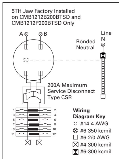
Figure 23. Catalog Numbers – CMB1212P200BTSD and CMB1212P200BTS
