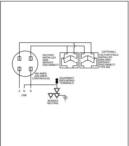
Figure 47. Type CH Wiring Diagram 4
