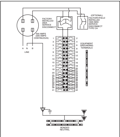
Figure 50. Type CH Wiring Diagram 7
