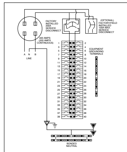
Figure 57. Type BR Wiring Diagram 5
