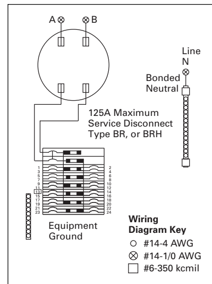
Figure 34. Catalog Numbers – MBE1224B125TS, MBE1224B125TF, MBE1224B100TS and MBE1224B100TF
