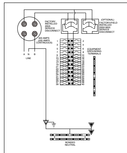
Figure 58. Type BR Wiring Diagram 6
