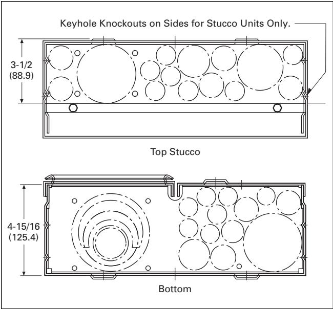
Figure 35. Knockouts for Stucco and Surface Units Catalog Numbers – CMBE3242B150BF, CMBE3242B200BF, CMBE3242B225BF, CMBE2222B100BF, CMBE2222B125BF, CMBE1212L200BF, MBE2040B200BF, MBE2040B150BF, MBE1428B100BF, MBE1428B125BF, MBE1212L200BF and MBE1836B125BF
