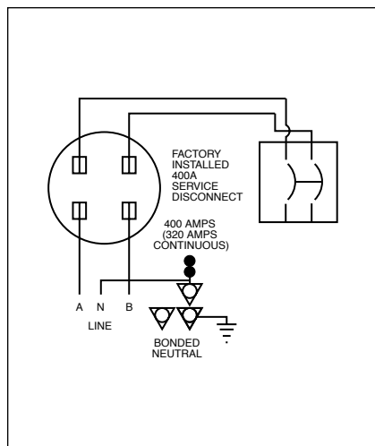
Figure 53. Type BR Wiring Diagram 1
