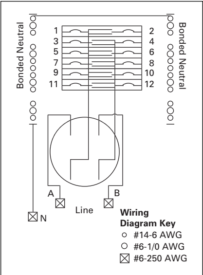
Figure 13. Catalog Numbers – MBE1212L200BS and MBE1212L200BF
