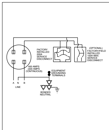
Figure 54. Type BR Wiring Diagram 2
