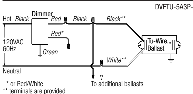
Wiring Diagram 10 Single-Pole Wiring
