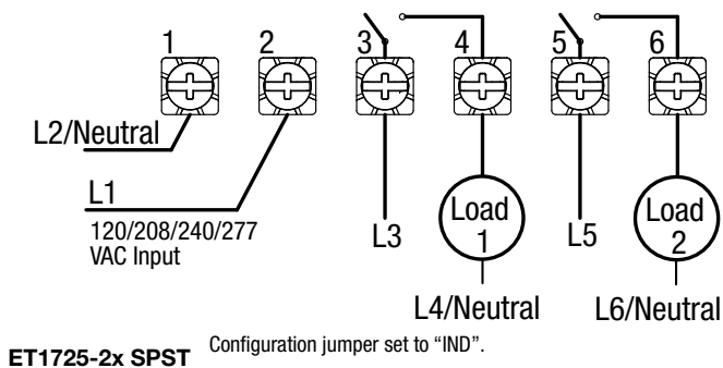
Timer Power
