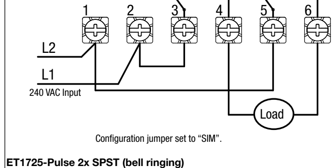
Timer Power
