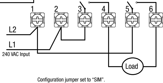
Timer Power
