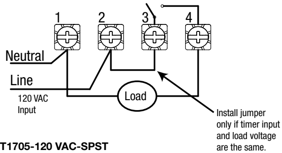
Timer Power
