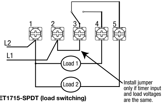
Timer Power
