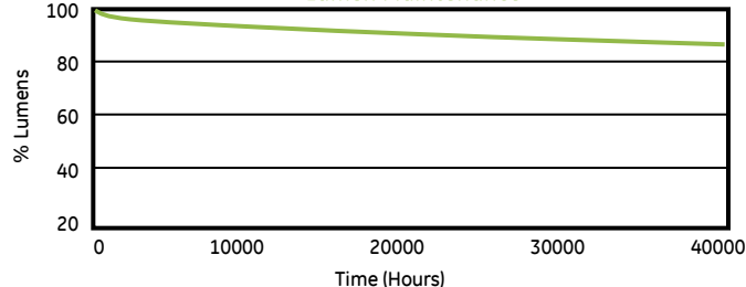
Lumen Maintenance
