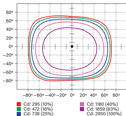
ISOCANDELA PLOT
