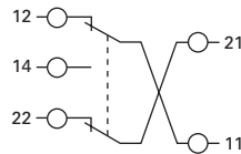
Wiring Diagram
