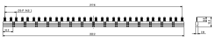
SV9Z-J232* Jumper for 14mm Relay
