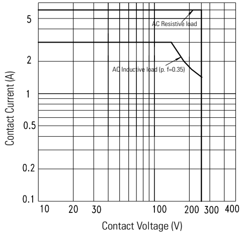
Maximum Switching Power AC
