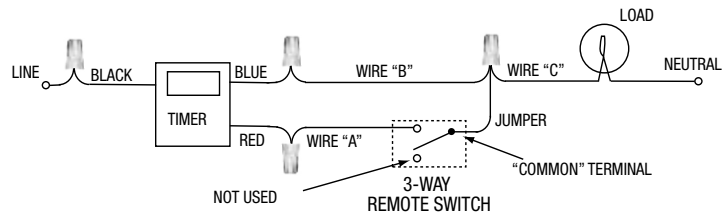
DIAGRAM 2: 2-SWITCH SETUP, TIMER INSTALL RE-USING EXISTING REMOTE 3-WAY SWITCH
